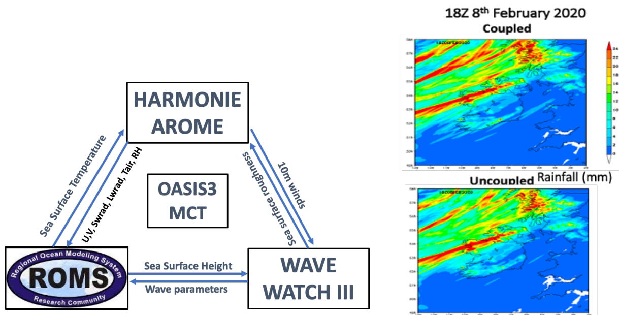
Figure 1: Flow diagram for fully coupled model (left panel); Rainfall comparison from Harmonie-AROME (uncoupled) with Harmonie-AROME-WW3 coupled model (right panel).
