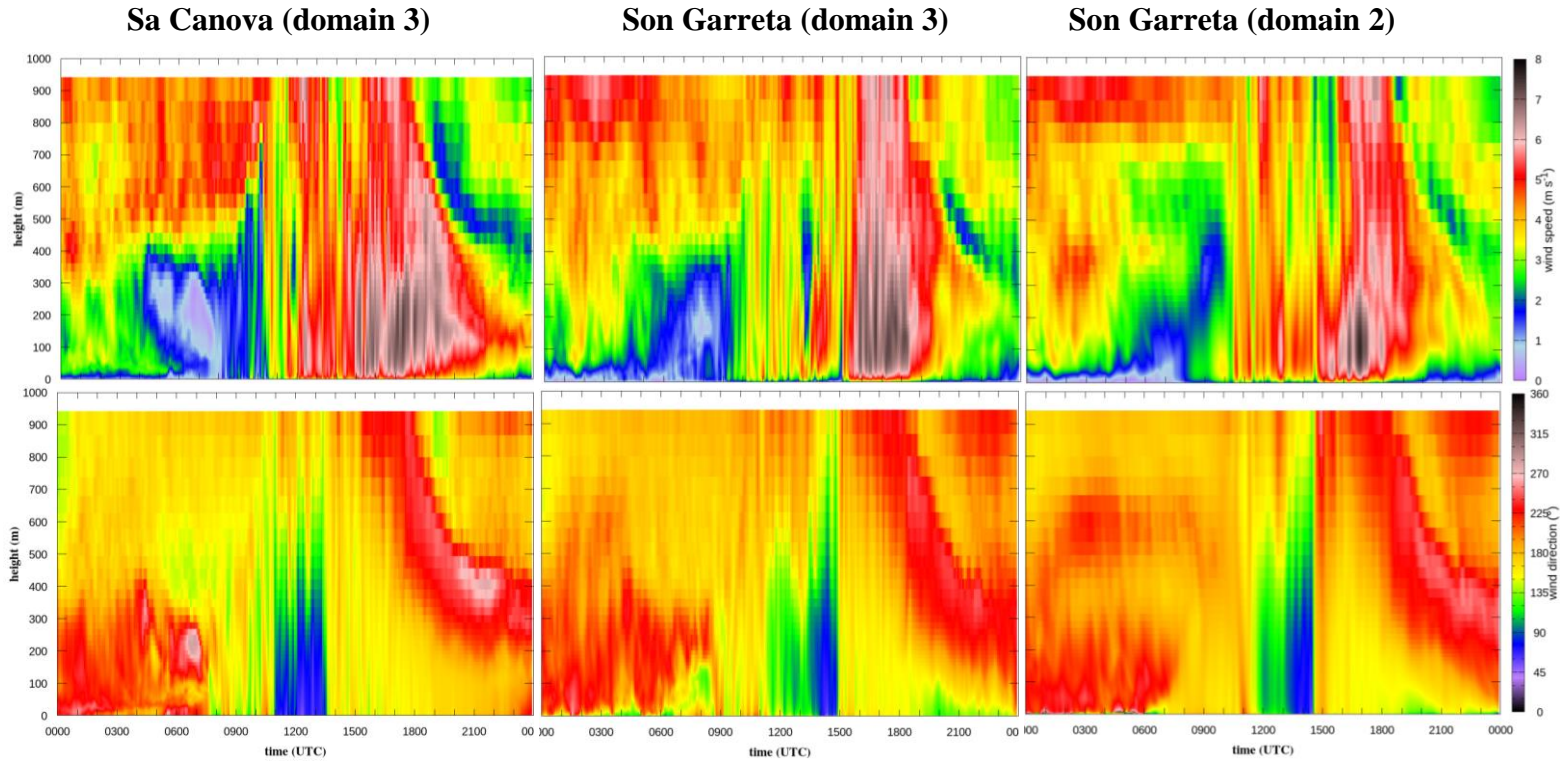
Figure 9. 24-h evolution of the vertical profiles (every 5min) obtained from the inner domain of the simulation (250m resolution, case 21 August 2021) at different sites: Sa Canova (labelled as SC in Figure 4) and Son Garreta (labelled as o in Figure 4). For the latter, the profiles obtained from the domain 2 (1km resolution) are also included.
